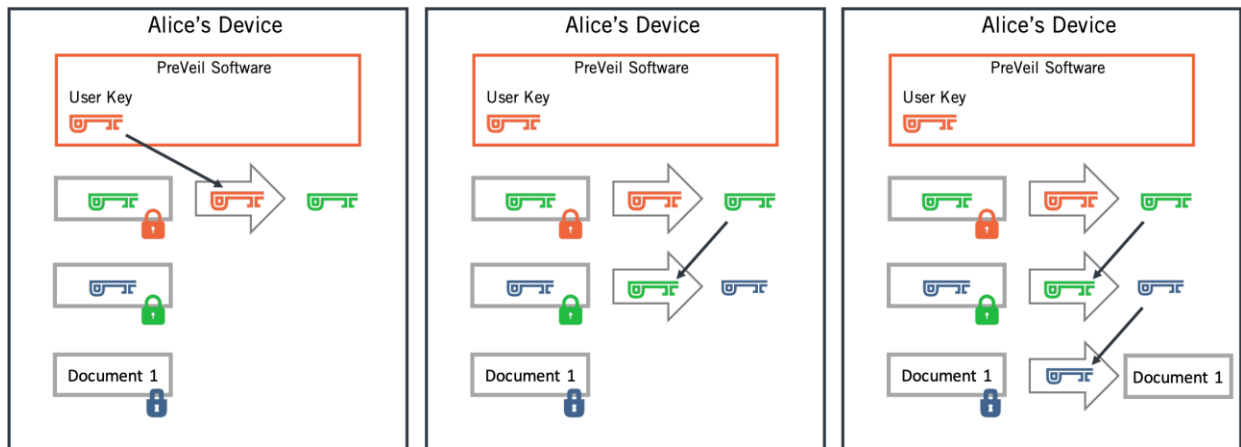
Figure 5 – After downloading all the files, the PreVeil software on Alice’s device first uses Alice’s orange private key (which is only kept on her devices) to decrypt the green Folder Read Key (left picture). The Folder Read Key is then used to decrypt the blue Document 1 decryption key (middle picture). The Document 1 decryption key is then used to decrypt Document 1 (right picture). This entire process happens automatically in the PreVeil software.
